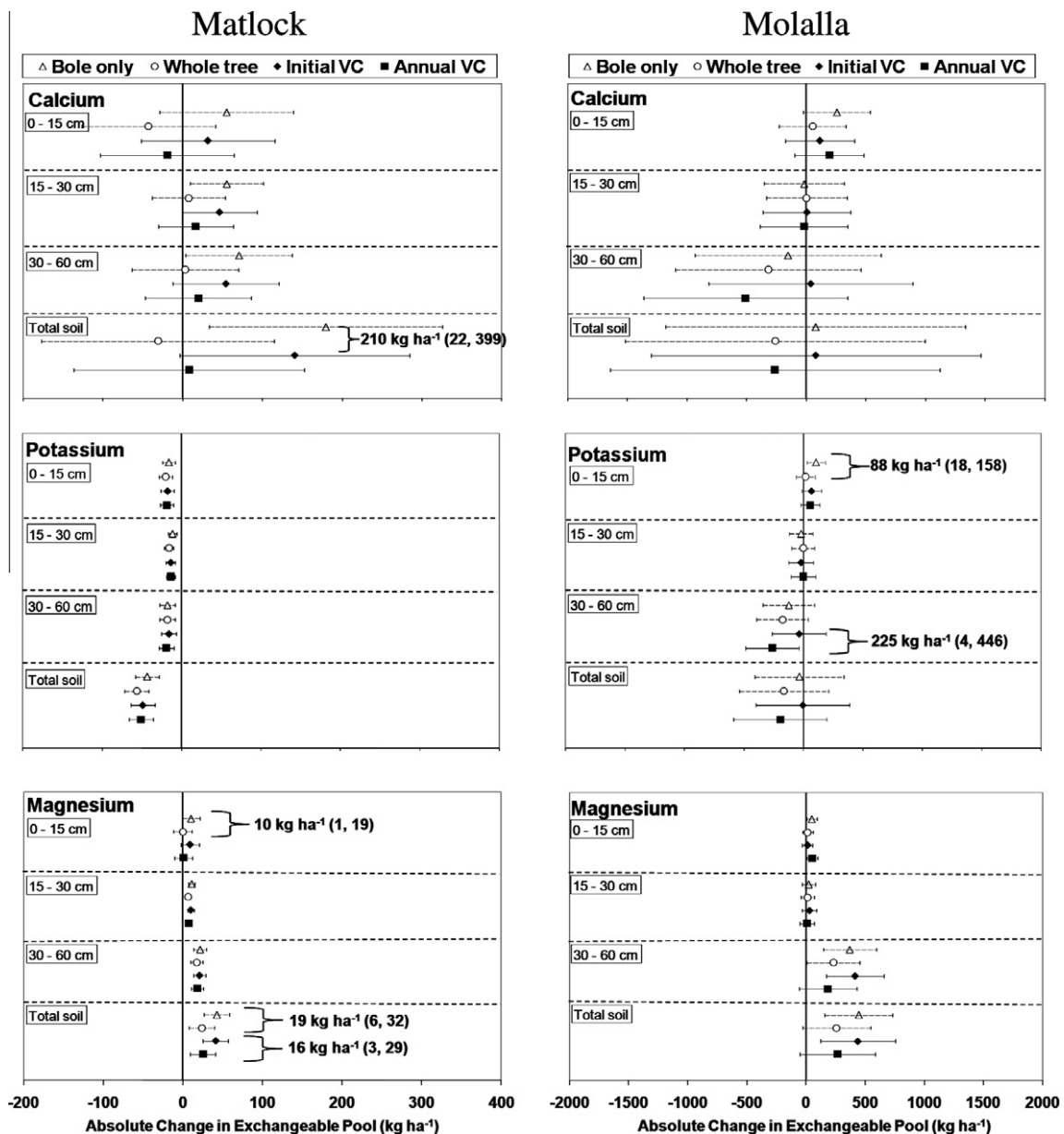
Fig. 2. Absolute change in exchangeable cations by treatment, depth, and site 5 years after forest harvest as affected by biomass removal and vegetation control. Error bars are the 90% confidence interval for each mean. Value next to a bracket when present is the estimated difference between treatments when significant effects occurred (90% CI in parenthesis).
