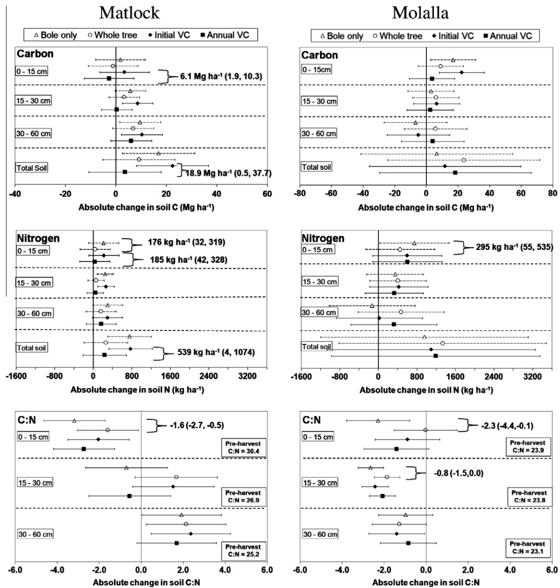
Fig. 1. Absolute change in soil C and N mass, and C:N by treatment, soil depth, and site 5 years after forest harvest as affected by biomass removal and vegetation control. Error bars are the 90% confidence interval for each mean. Value next to a bracket when present is the estimated difference between treatments when significant effects occurred (associated 90% CI in parenthesis). Note difference in scale among panels.
